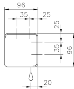
All fixing holes 2.5mm diameter
